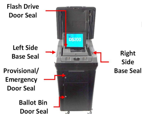
DS200 Tabulator/Scanner
