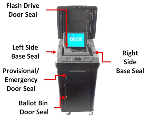
DS200 Tabulator/Scanner
